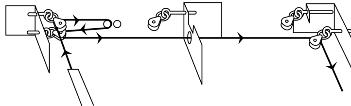
Non-Motor side rope routing
